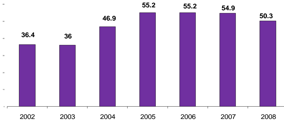
NEW YORK STATE, ANNUAL GAS PRODUCTION, Bcf
